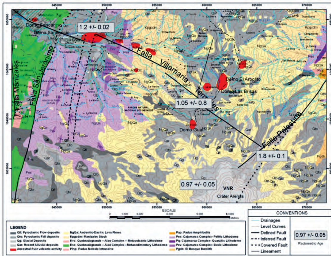
Figure 7. Geological map of the NRV showing its location at the intersection of the Villa María-Termales and Palestina faults. Map modified from Toro et al. (2010) with radiometric ages from Thouret et al. (1990).
