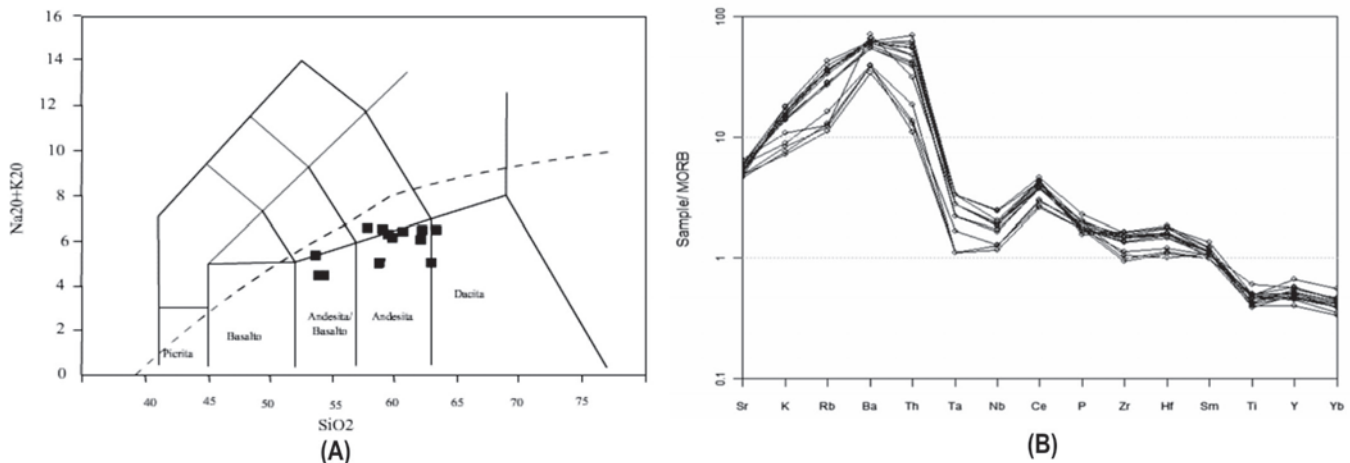
Figure 14. (A) TAS diagram (B) Aracnogram of the Ancestral Ruiz stage volcanic rocks.
