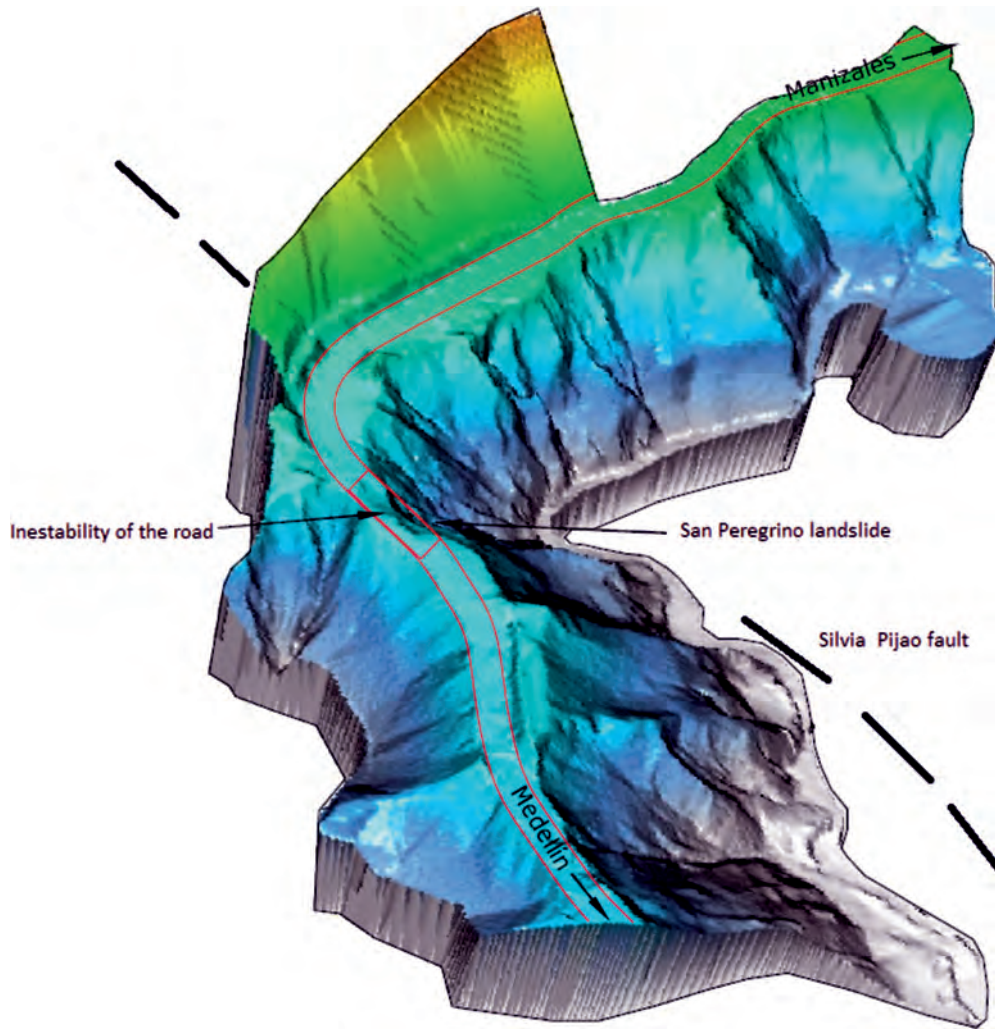
Figure 25. Geomorphologic expression of the Silvia - Pijao fault in San Peregrino. Active tectonics generates instabilities along the roadway connecting Manizales and Medellin. One lane of the road has been damaged and a new bridge was necessary to keep the road open. Modified from Estrada et al. (2009).
