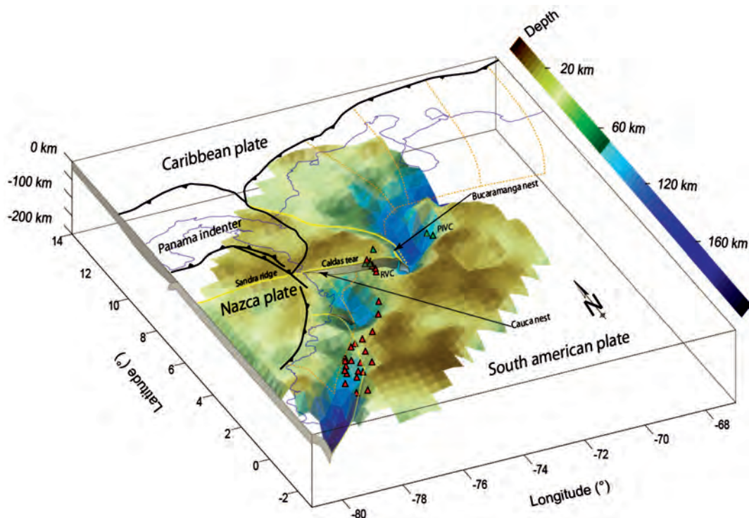
Figure 4 Top surface of subducted slabs beneath northwestern South America estimated from hypocentral distribution of about 68,000 local earthquakes located by the Colombian seismic network (CNSN). A 3D surface was defined by earthquakes and constrains the presence of subducted slabs beneath northwestern South America.
