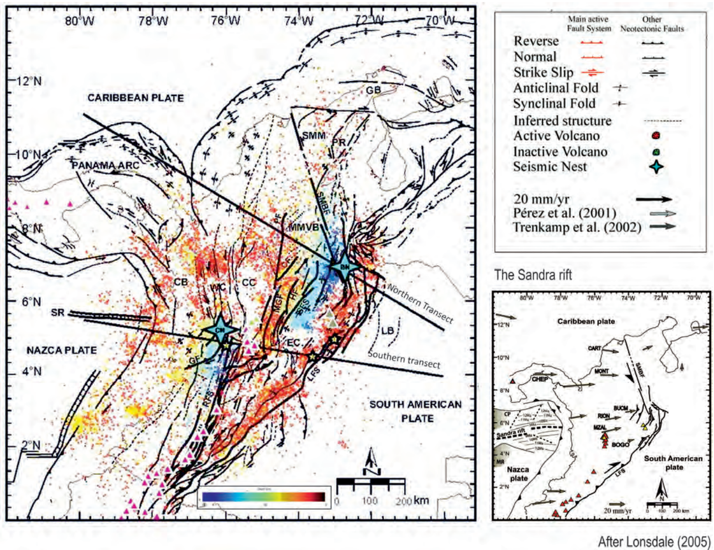
Figure 1. Tectonic setting of Colombia and Panama. Map shows principal plate boundaries, fault systems and neotectonic faults, as well lineaments (dashed lines) and other smaller faults (thin lines). Dots represent hypocentral distribution of the approximately 68,000 earthquakes 1.0 = m_L > 6.7 located by the CNSN between 1993 and 2008. Color scale, continuously varying, indicates the depth of events. Arrows represent station velocity GPS vectors relative to stable South America. CHEP and BOGO denote the GPS's stations used as reference to estimate the onset of the Panama-arc and South American plate collision. Other GPS stations in the Panama-arc collision area are MANZ, RION, BUCM, MONT and CART. The northern and southern profiles are tomographic sections described in this study. Key to abbreviations: SMM, Santa Marta massive; Choco block, CB; Western Cordillera, WC; Central Cordillera, CC; Eastern Cordillera, EC; Perija range, PR; Guajira basin, GB; Llanos foreland basin, LB; Middle Magdalena Valley basin, MMVB; Romeral fault system, RFS; Santa Marta-Bucaramanga fault, SMBF; Palestina fault, PF; Cimitarra fault, CF; Mulato-Getudo fault, MGF; Honda fault, HF; Salinas fault system, SFS; Garrapatas fault, GF; Llanos Fault System, LFS; Ibaguè fault, IF; Sandra rift, SR; Bucaramanga nest, BN; Cauca nest, CN; Paipa - Iza volcanic complex, PIVC; Ruiz volcanic complex, RVC. Yellow stars correspond to the Tauramena earthquake (Jan. 19 th , 1995, M_w=6.5 ), Armenia earthquake (Jan. 25 th , 1999, M_w=6.2 ) and Quetame earthquake (May 24 th , 2008, m_L=5.7 ).
