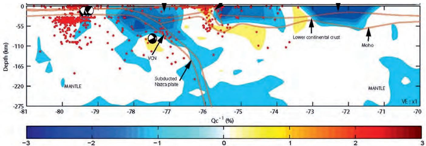
Figure 3. Tomographic section along the southern transect. Coda-wave attenuation anomalies showing the subduction geometry of the Nazca plate. Transect crosses the southern part of the Panama arc/indenter and the Cauca earthquake nest.
