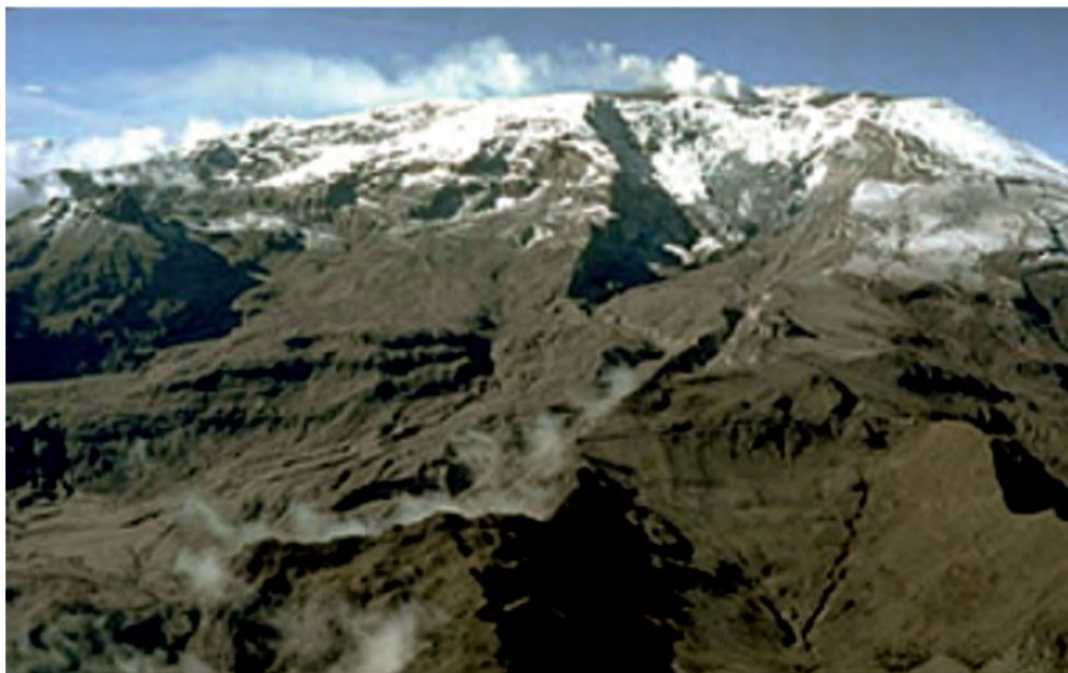
Figure 19. The horseshoe-shaped amphitheatre of Azufrado River produced by collapse of the Northern face of VNR approximately 3100 years B.P. (Thouret et al. , 1990). The headwaters is located near the active Arenas crater with the small fumarole. This geomorphic feature resembles the Mt St Helens volcano (US) following its May, 1980, eruption. Photo credit: USGS (Janda, 1985).
