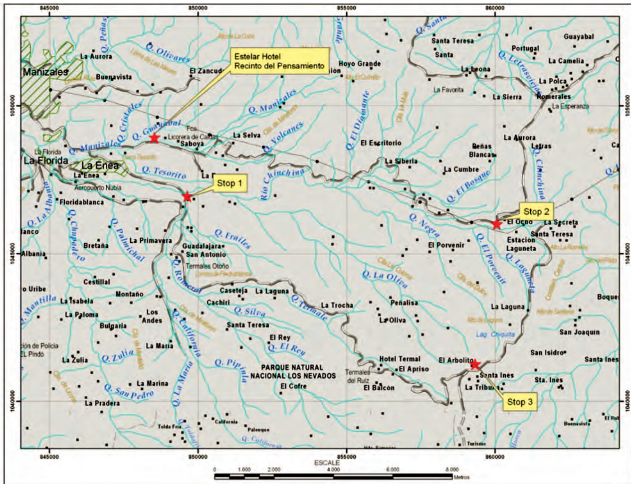
Figure 9. Location of departure site in Manizales and locations of Stops 1 to 3.
