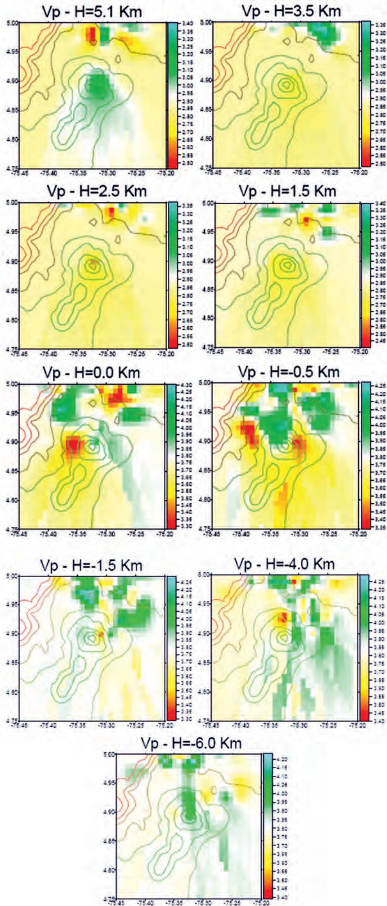
Figure 8. \%V_p -tomograms estimates constructed using first P-arrivals from local earthquakes near the NRV (Vargas et al. , 2000).
