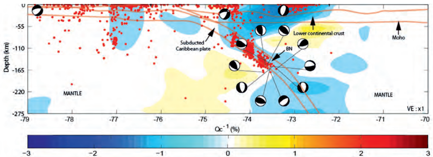
Figure 2. Tomographic section along the northern transect. Coda-wave attenuation anomalies supporting the dip changes in the subducted slab.
