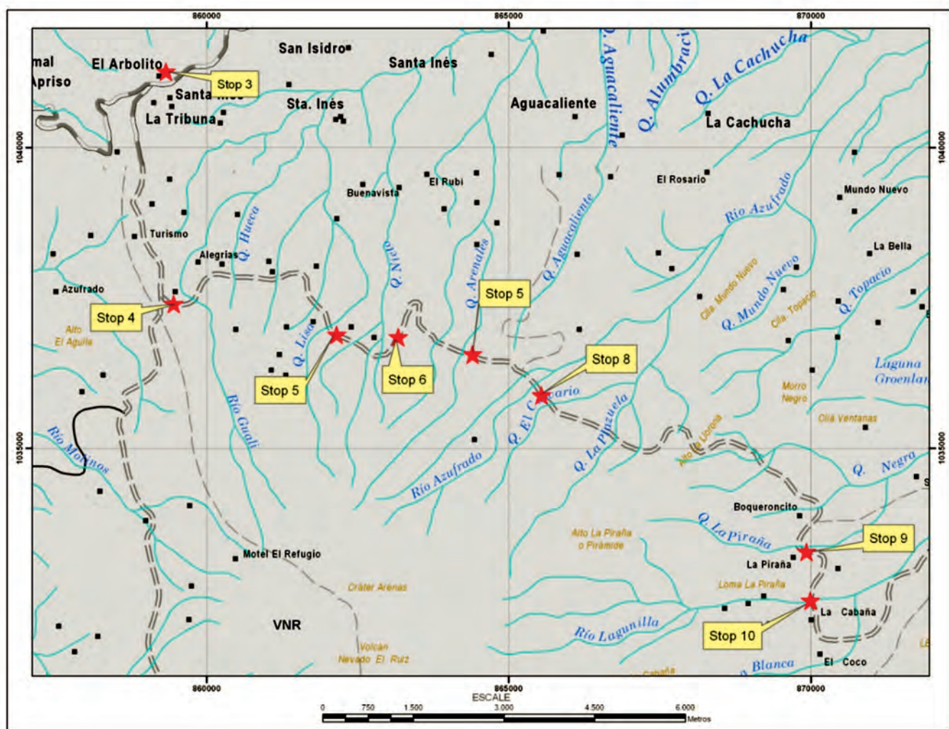
Figure 10. Location Stops 3 to 10, following the dirt road La Esperanza-Murillo.
