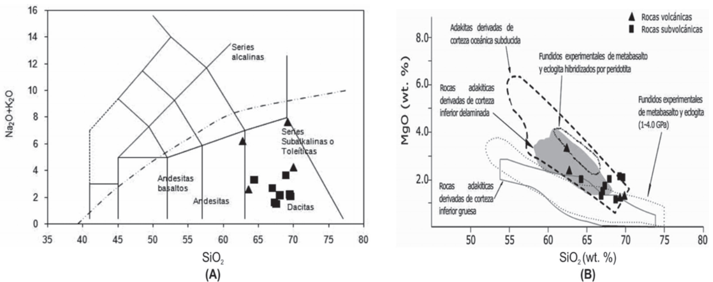
Figure 12. (A) TAS diagram. (B) MgO vs. \text{SiO}_2 Harker diagram showing the compositions of volcanic rocks southeast of Manizales (both figures from Toro et al. , 2008).
