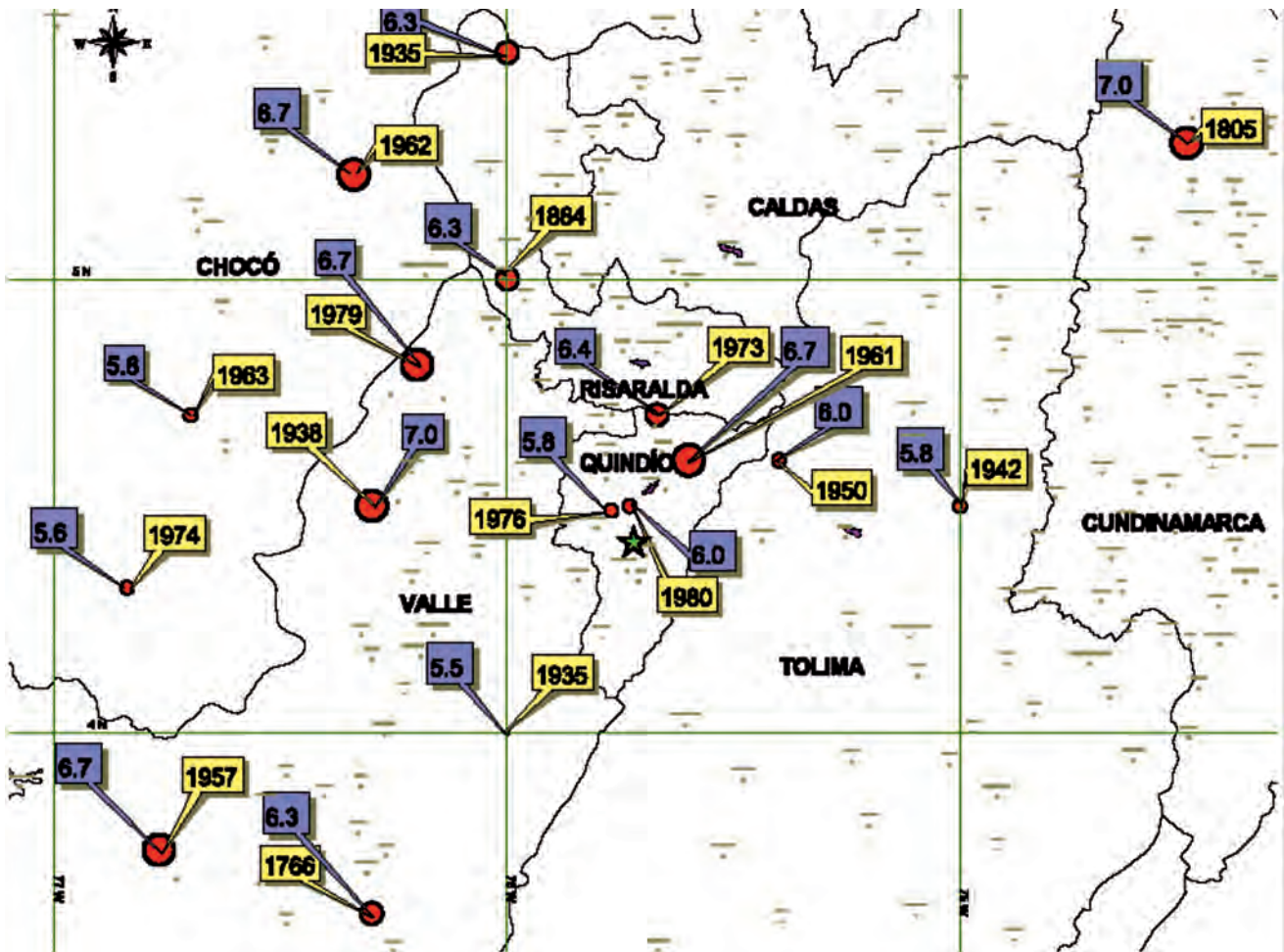
Figure 30. Historical record of strong motion events in the "Eje Cafetero" region. Taken from INGEOMINAS webpage: www.ingeminas.gov.co
