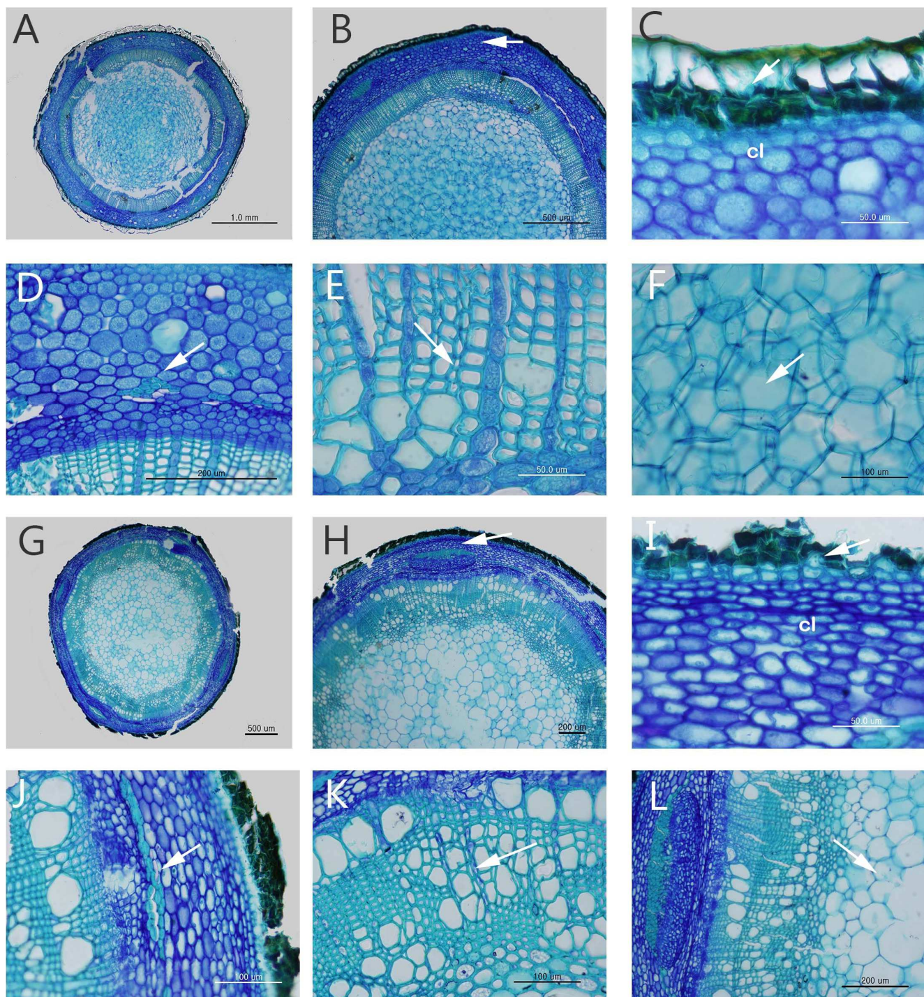
Figure 1. Calycanthus occidentalis (A-F); A. Cross section of young stem, B. A detail portion of cross section (arrow head shows the vascular bundle), C. Epidermis and collenchyma (arrow head represent epidermis, and cl shows collenchyma), D. Sclerenchyma with the colony, E. Tracheid and vessel, F. Pith. Chimonanthus praecox (G-H); G. Cross section of young stem, H. A detail portion of cross section (arrow head shows the vascular bundle), I. Epidermis and collenchyma (arrow head represents epidermis, and cl shows collenchyma), J. Sclerenchyma with the colony, K. Tracheid and vessel, L. Pith.
