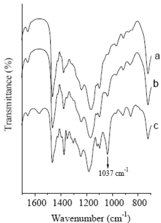
Figure 3 – Spectrum in the IV region of Biodiesel: (a) soybean oil; (b) biodiesel obtained with 10% of NaNb500 catalyzer (reflux); (c) standard biodiesel.
