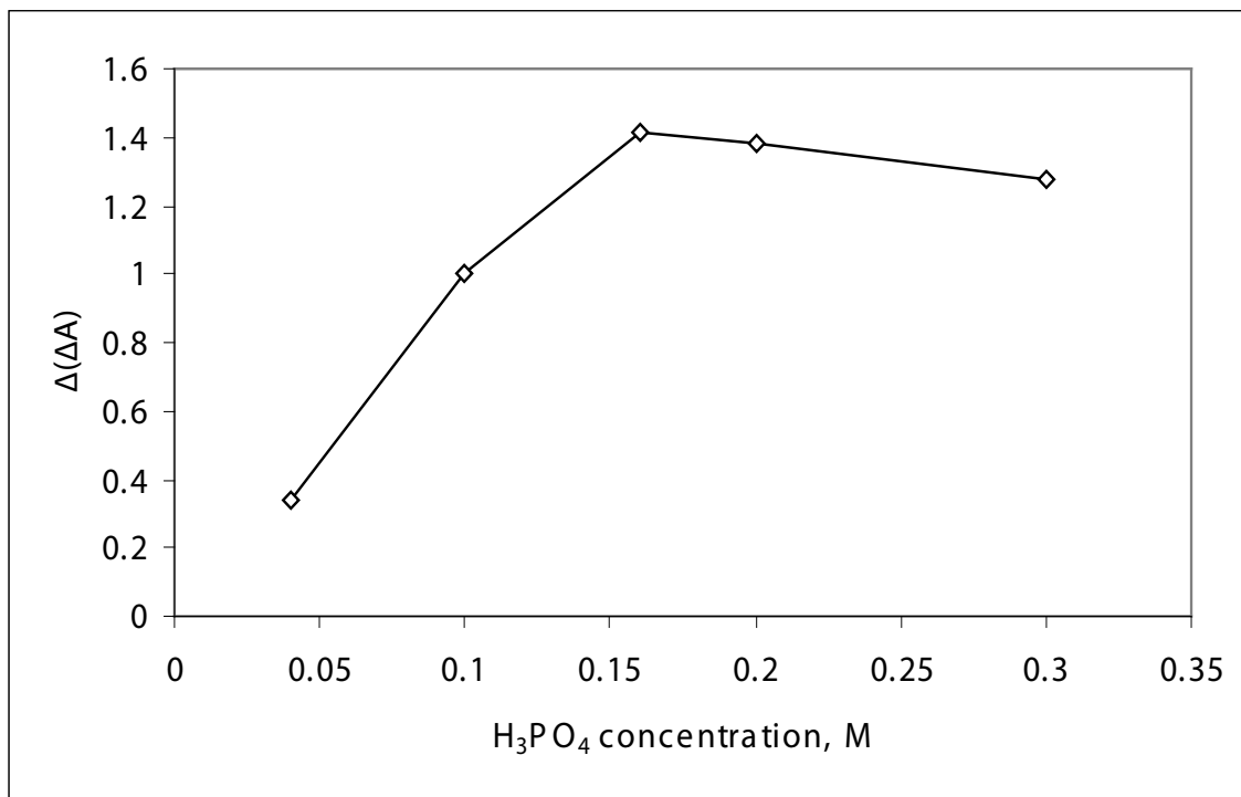
Fig.1. Effect of \text{H}_3\text{PO}_4 concentration on analytical sensitivity.[Optimum conditions: 1 \times 10^{-4} \text{ mol L}^{-1} Ponceau Xylidine, 9 ppb \text{V}(\text{V}) , 2 \times 10^{-4} \text{ mol L}^{-1} SSA and 1 \times 10^{-3} \text{ mol L}^{-1} \text{BrO}_3^- at 640 nm and 25^\circ\text{C} for the fixed-time method of 7 min]
