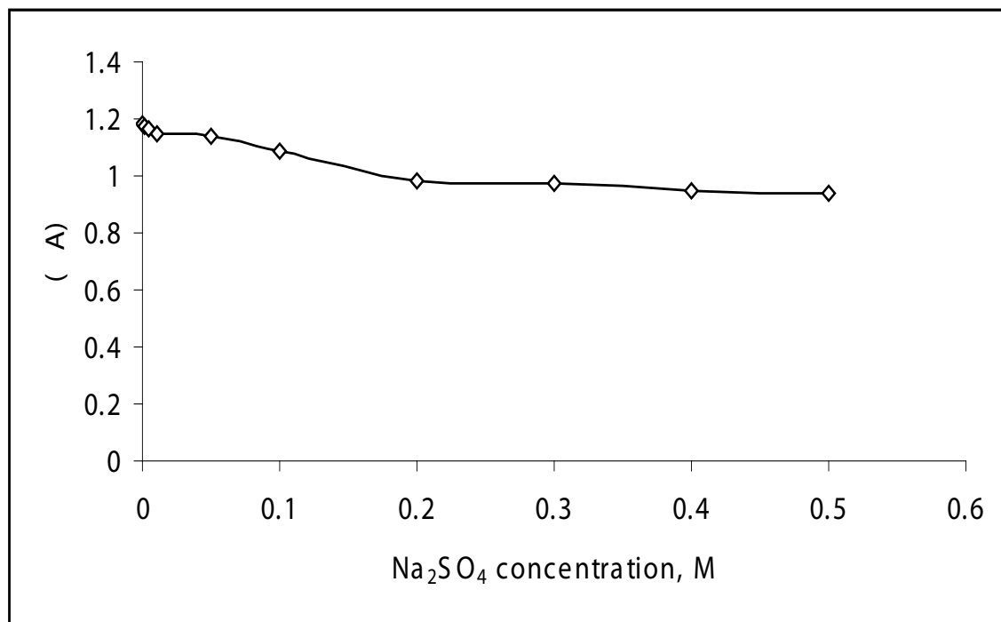
Fig.5. Effect of ionic strength on analytical sensitivity.[Optimum conditions: 6 \times 10^{-4} mol L -1 Ponceau Xyldine, 0.015 mol L -1 BrO 3 - , 6 \times 10^{-4} mol L -1 SSA, 9 ppb V(V) and 0.16 mol L -1 H 3 PO 4 at 640 nm and 25°C for the fixed-time method of 7 min]
