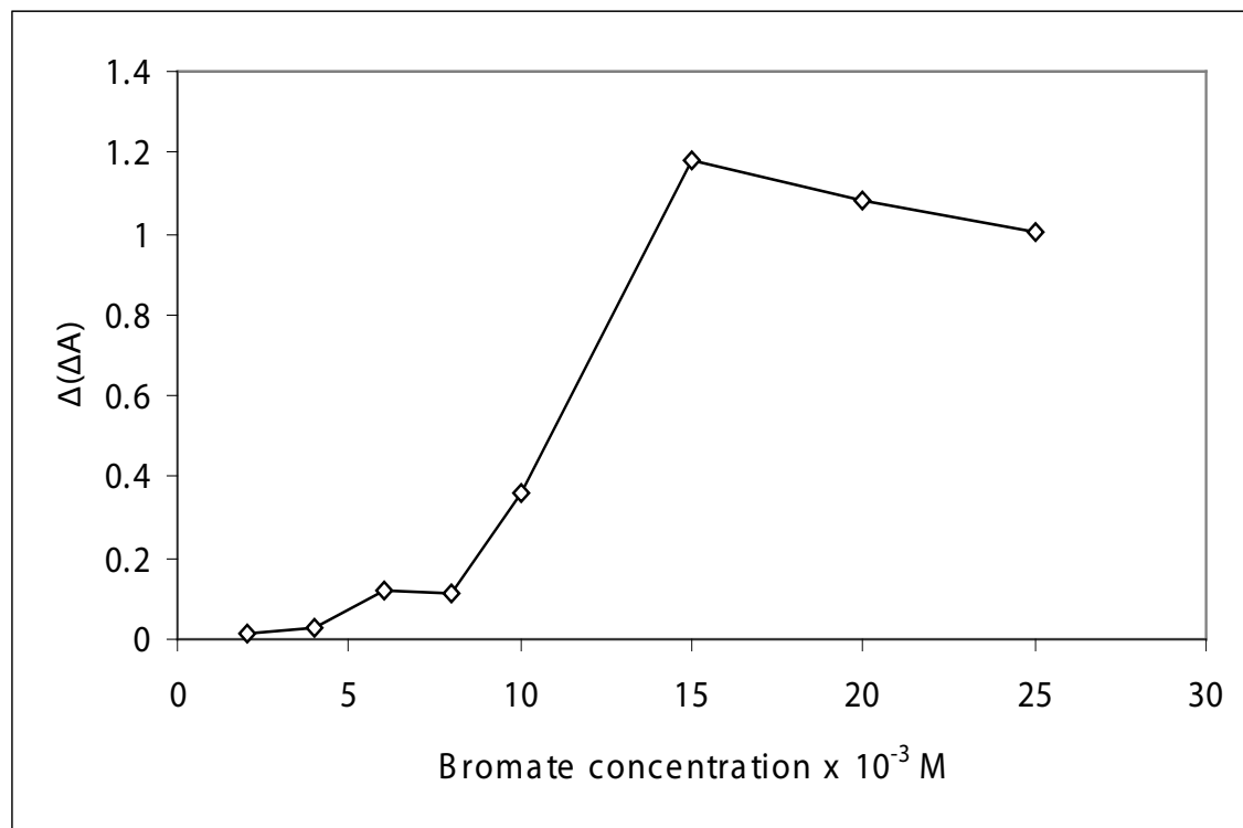
Fig.2. Effect of bromate concentration on analytical sensitivity.[Optimum conditions: 1 \times 10^{-4} mol L -1 Ponceau Xylidine, 9 ppb V(V), 2 \times 10^{-4} mol L -1 SSA and 0.16 mol L -1 H 3 PO 4 at 640 nm and 25°C for the fixed-time method of 7 min]
