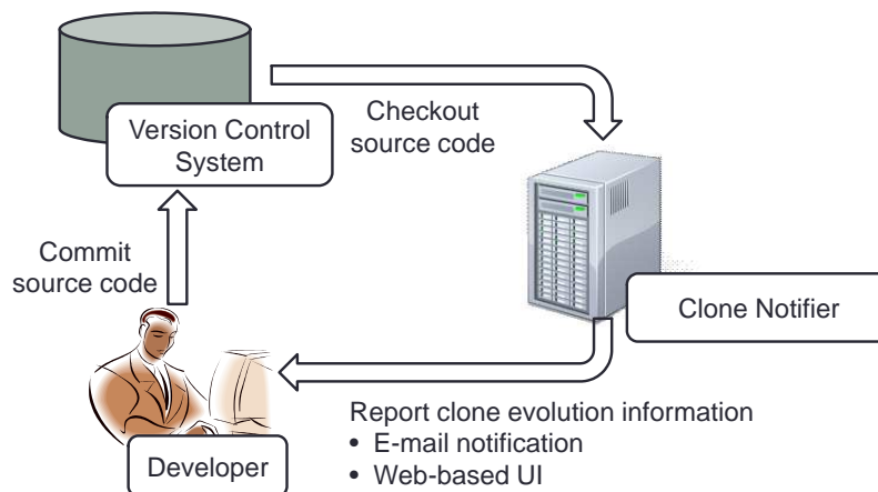
Figure 1: An Overview of Clone Notifier
