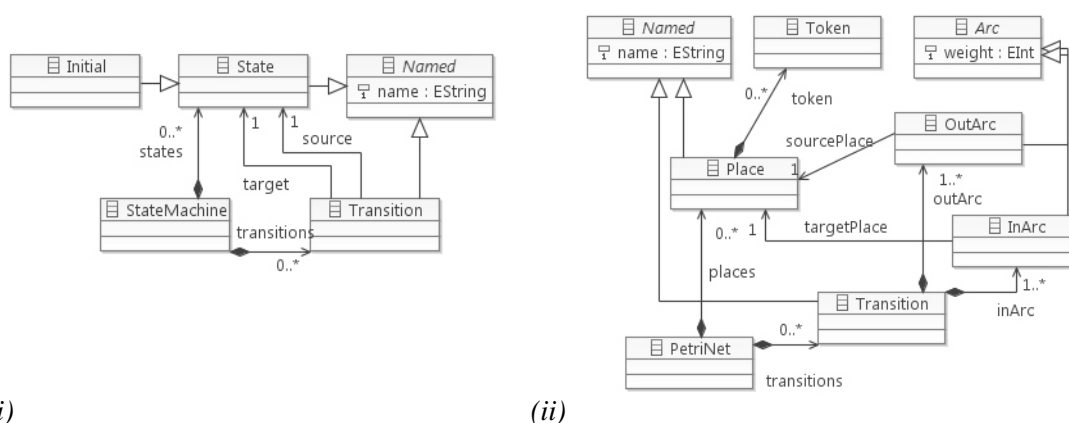
Figure 2: The State Machine Language Metamodel (i), and the PetriNet Language Metamodel (ii)
