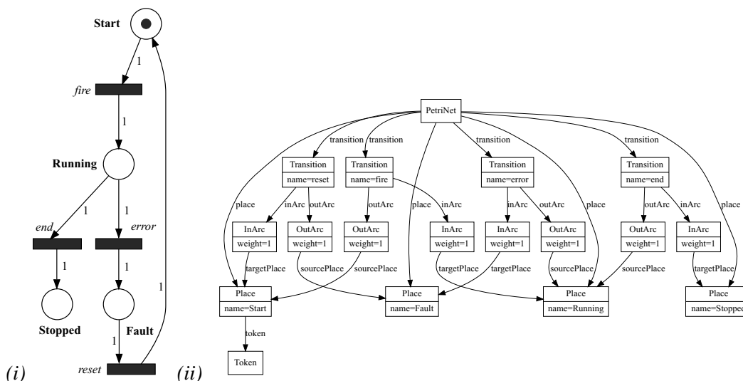
Figure 4: The standard visual representation of a petri net using the language’s concrete syntax (i), and its internal hierarchical EMF representation (ii): a sentence instance of the petri nets metamodel. There exists very efficient verification algorithms/techniques developed to determine invariants of a petri net sentence, such as the overall number of tokens.
