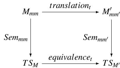
Figure 1: A commutative diagram illustrating the logical principles of the approach. M and M' are representative sentences from source and target languages of the translation. These representative sentences that can be extracted from a translation specification, where mm and mm' are metamodels identifying each language, \text{Sem}_{mm} and \text{Sem}_{mm'} are each one a set of SOS rules defined for each language, and \text{TransitionSystem}_M and \text{TransitionSystem}_{M'} are the resulting transition system from each sentence M and M' respectively.
