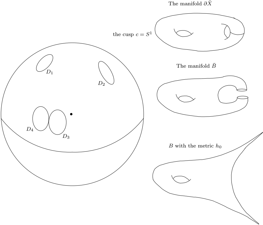
Figure 1: The infinity B of the quotient X = \Gamma \backslash \mathbb{H}^3 where \Gamma is a Schottky group gluing D_3 \longleftrightarrow D_4 and D_1 \longleftrightarrow D_2 ; \bar{B} is a manifold with fibred boundary.
