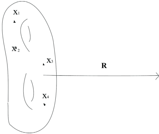
Fig. 1: (x_1, \dots, x_4) -marked points
