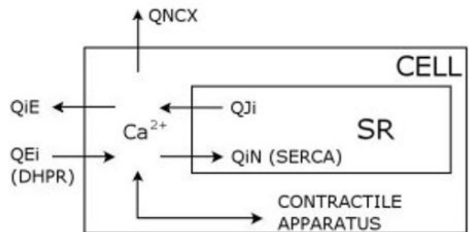
Fig. 1: Some Ca^{2+} transport mechanisms in heart cell
