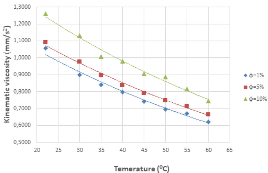
FIGURE 4. Change in viscosity with rise in temperature.
