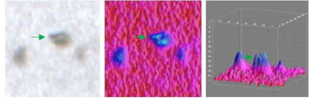
FIGURE 3. Identification of emulsion defects by surface plots and 3D imaging. The image size is approximately 0.6 \times 0.6 mm.
