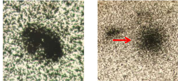
FIGURE 4. Detailed analyses with the Sonneberg Observatory Zeiss Microscope: Emulsion defect (left) and real OT image (right). The image size is \sim 0.3 \times 0.3 mm.
