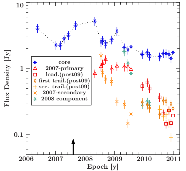
Fig. 4: Flux density evolution of the "core" region and the components as a function of time. Conservative errors of 15% are assumed for the flux densities of the model-fit components. The component symbols are the same as in Figure 3 with the addition of the "core" region, represented by stars. The black arrow at the bottom indicates the calculated and almost identical ejection date of the primary and secondary component based on the derived jet kinematics
