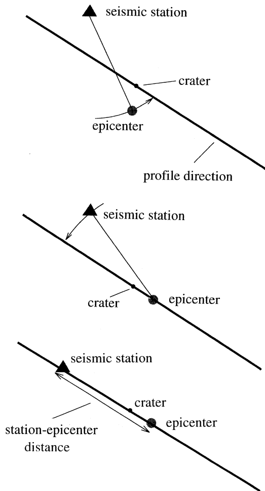
Fig. 6. Description of the procedure applied to project ray paths and earthquake sources/stations on the vertical plane profile.
