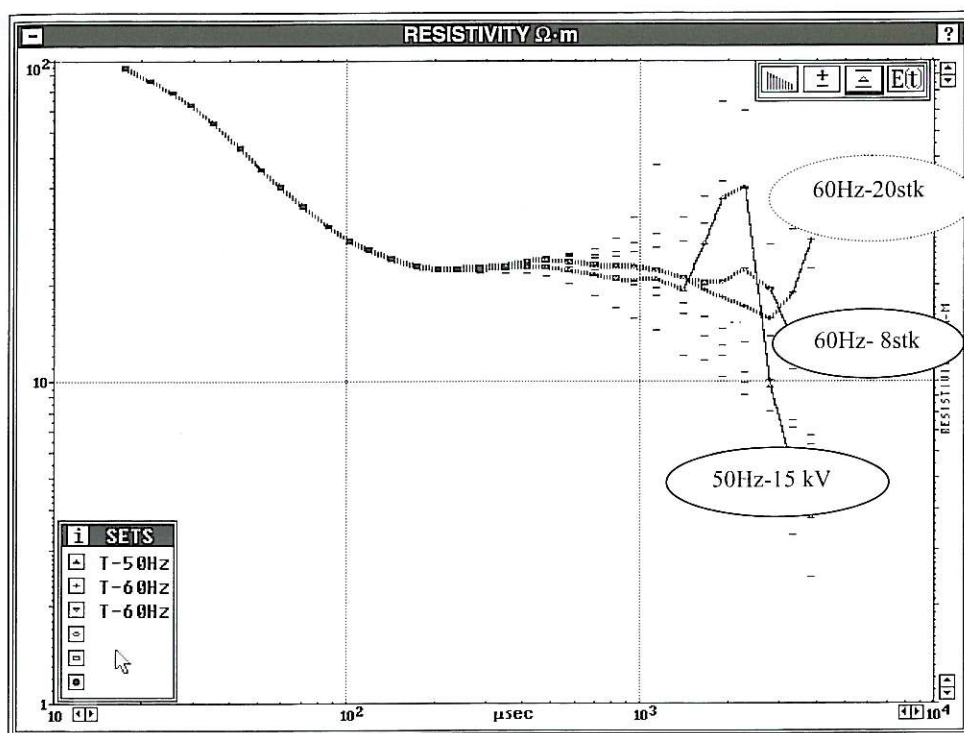
Fig. 8. Effect of an electrical power line with different acquisition (by courtesy of AEMR - The Netherlands).
