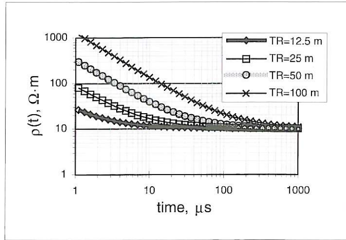
Fig. 5. Apparent resistivity versus time for different loop size in 10- \Omega \cdot \text{m} homogeneous half space (by courtesy of AEMR - The Netherlands).
