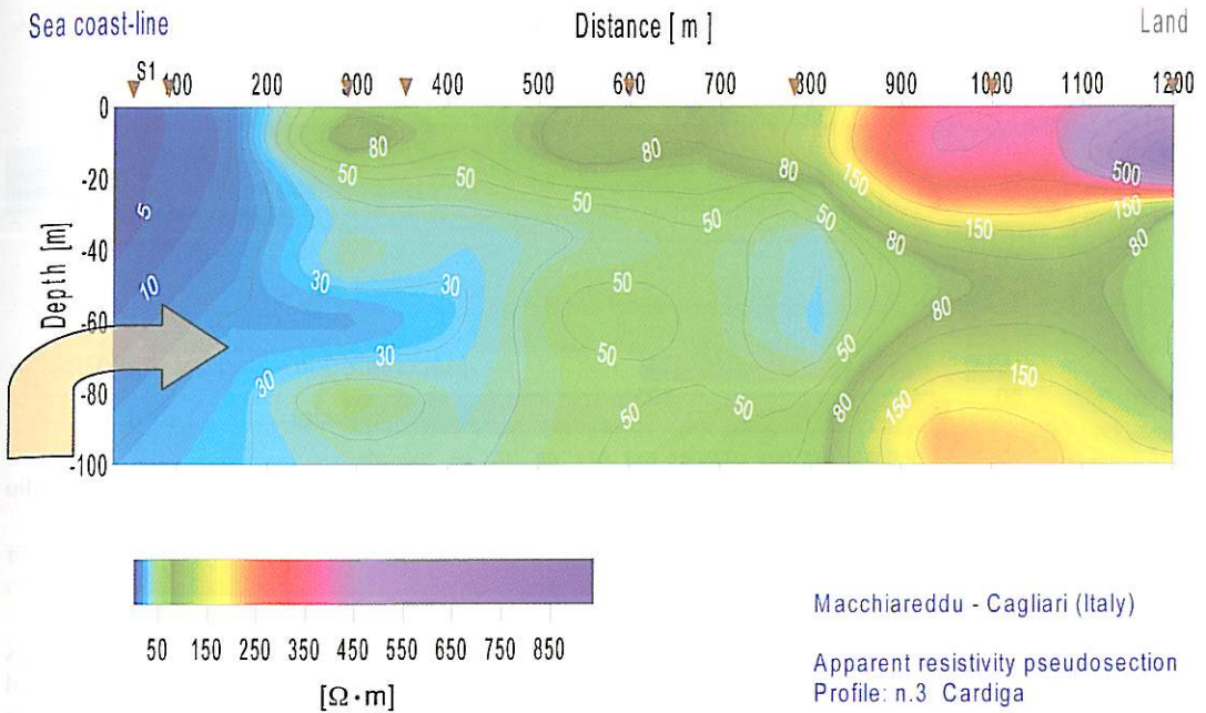
Fig. 11. Apparent resistivity pseudosection perpendicular to the coast line, showing the salt water intrusion to 800 m from the sea (after Godio et al. , 1999).
