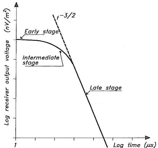
Fig. 4. Receiver output voltage versus time.
