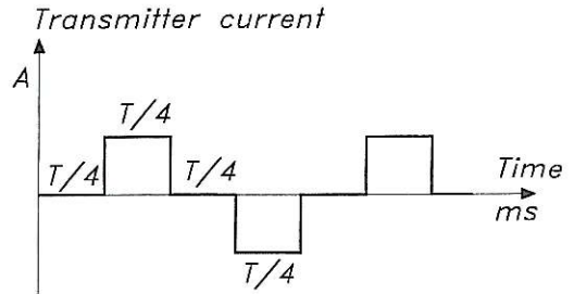
Fig. 1. Transmitter current waveform.
