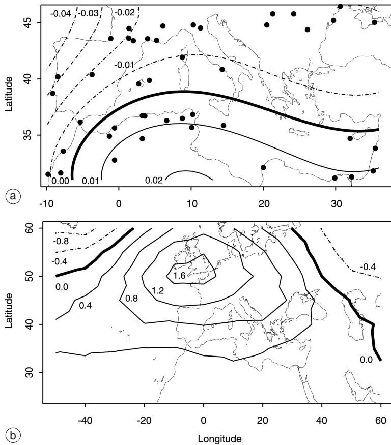
Fig. 4a,b. a) The geographical form of the first precipitation canonical function. The contours indicate equal loading values. Increasing loading values represent increased correlation between the variations of precipitation at that locality and the pressure field. b) The geographical extent of the first pressure canonical function. The contours indicate equal loading values. Increasing loading values represent increased correlation between the variations of pressure at that locality and the whole precipitation field. Thus regions of high loading are particularly responsive. N.B. : the loading values in a) and b) are not directly comparable due to the choice of normalisation (see text for further details).
