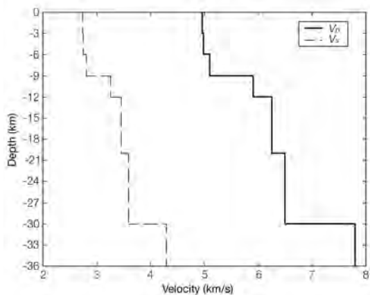
Fig. 5. Local velocity model.
