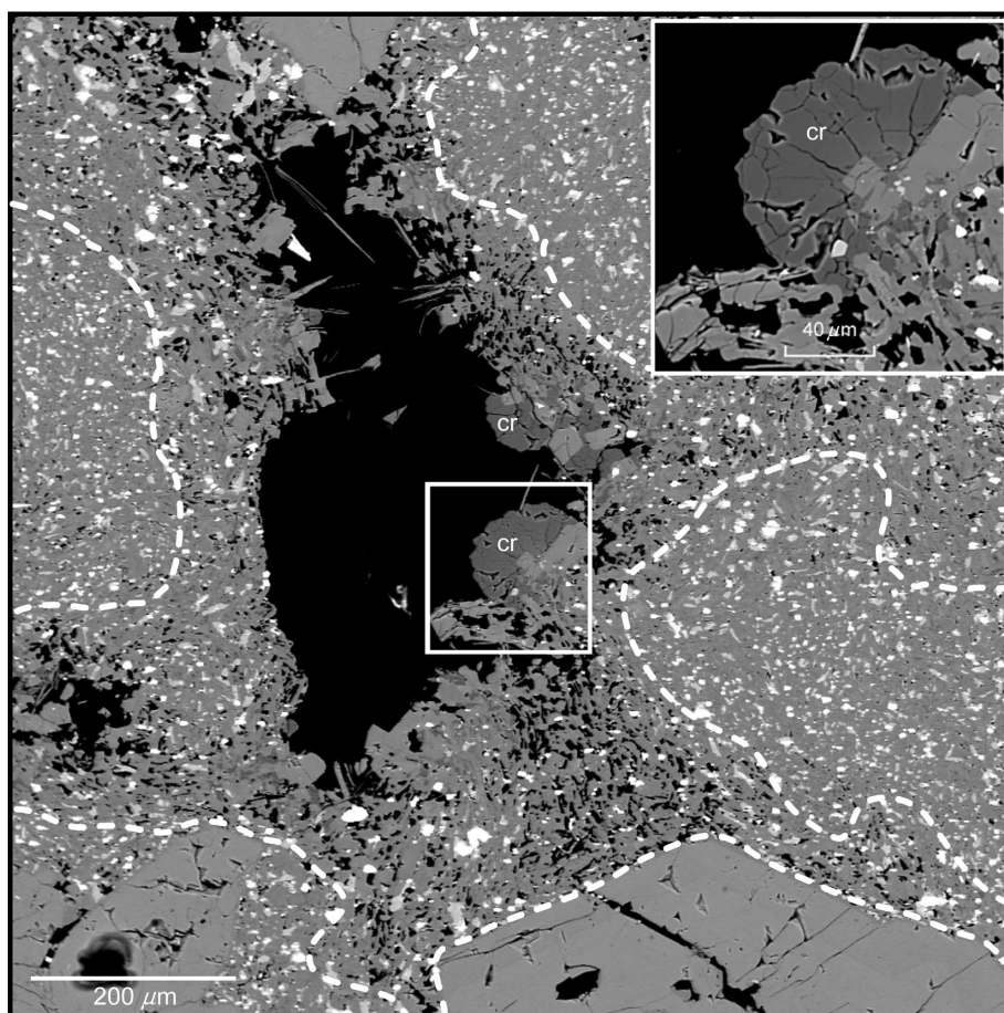
Fig. 1. Back-scatter electron images of a vesicle filling containing several patches of crystalline silica (cr), inferred to be cristobalite. The dashed lines indicate the approximate outline of the vesicle and interconnecting veins before the vesicle-filling assemblage was formed. Note the radial growth texture of the silica patches. The small needles sticking into the open space are F-phlogopite. Inset shows detail of one of the silica patches.
