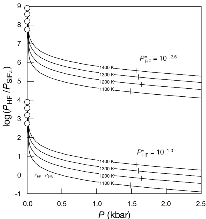
Fig. 3. Variation of \log(P_{\text{HF}}/P_{\text{SiF}_4}) with total pressure for various temperatures at P_{\text{HF}}^* = 10^{-2.5} and P_{\text{HF}}^* = 10^{-1.0} , respectively. The importance of SiF 4 increases with decreasing temperature, increasing P_{\text{HF}} , and increasing pressure. The circles represent data at 1 bar, and are equivalent to the values in fig. 2 at the same temperature and P_{\text{HF}}^* .
