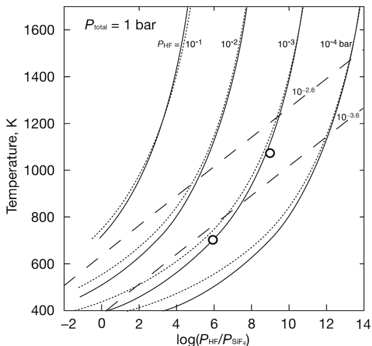
Fig. 2. Variation of \text{SiF}_4/\text{HF} (expressed as \log[P_{\text{HF}}/P_{\text{SiF}_4}] ) with T (in K) at different partial pressures of HF, and 1 bar total vapour pressure ( P_{\text{HF}}+P_{\text{SiF}_4}+P_{\text{H}_2\text{O}} = 1 ). Continuous lines are from our own calculations, whereas dotted lines are data from Rosenberg (1973), dashed lines are after White and Hochella (1993), and the two circles are data points from Symonds et al. (1992) with P_{\text{HF}} = 10^{-3.07} bar. Uncertainties in our data due to uncertainties in heat of formation and enthalpy of \text{SiO}_2 , HF, \text{H}_2\text{O} and \text{SiF}_4 are about 25^\circ and 0.2 log units. Note that the relative importance of \text{SiF}_4 increases both with total amount of F in the system ( i.e. , P_{\text{HF}} ), and with decreasing temperature. White and Hochella (1992) trends are clearly offset and predict HF/ \text{SiF}_4 variations with temperature that are much larger than other models.
