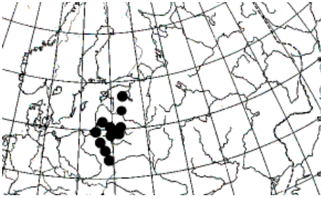
Fig. 3. Distribution of Verrucaria praetermissa in Eastern and East Central Europe ● modern records
