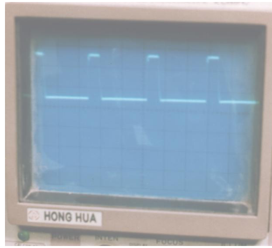
Quasi-Square Waveform, Frequency =250 kHz
