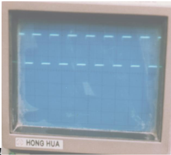
Square Waveform, Frequency =160 kHz
