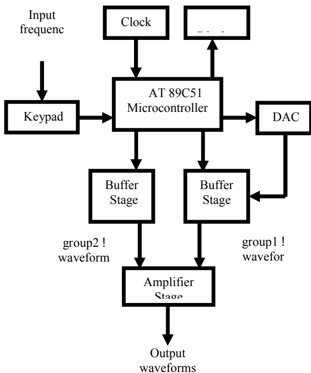
!!Figure 1: Hardware-based scheme
