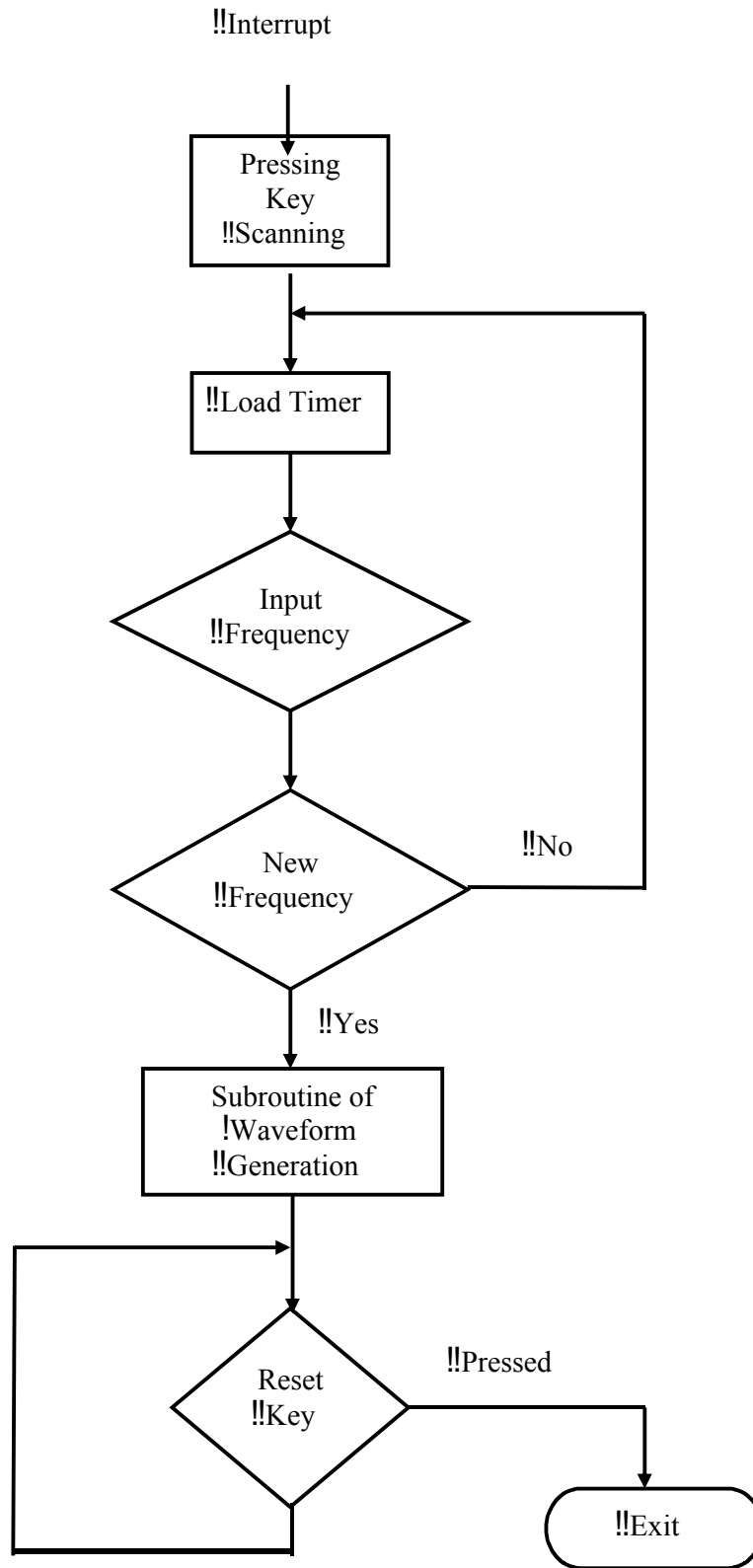
!(b): Interrupt Service Routine Program (ISR)
