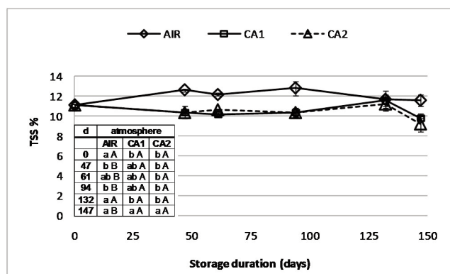
Fig. 2 - Changes in blueberry soluble solid content during cold storage ( 0^{\circ}\text{C} ) in different atmosphere regimes (Air; CA1= 4 kPa \text{O}_2 and 10 kPa \text{CO}_2 ; CA2= 2 kPa \text{O}_2 and 9 kPa \text{CO}_2 ). Values are mean \pm SE of triplicate samples. In the table, different lowercase letters indicate significant differences among values after different storage periods at each atmosphere regime and different capital letters indicate significant differences among values at different atmosphere regimes, at each sampling time ( P \leq 0.05 ).
