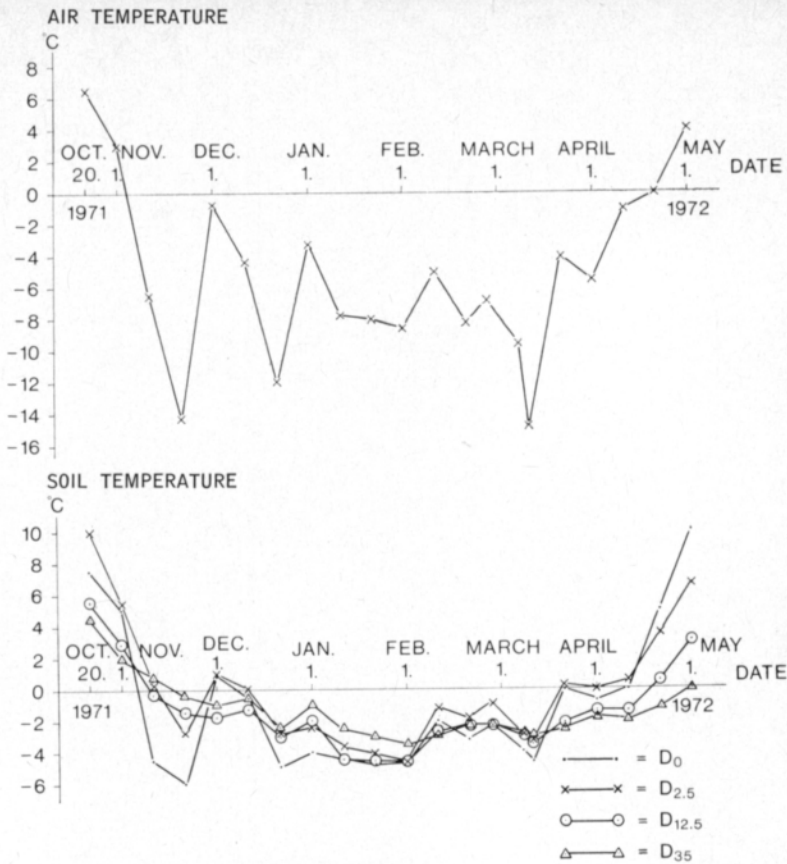
Fig. 1. Air and soil surface temperatures measured in the experimental field of Kiikala in the winter 1971–1972. D_0 = depth of measurement 0 cm, D_{2.5} = 2.5 cm, D_{12.5} = 12.5 cm and D_{35} = 35.0 cm. The values given, represent the mean values of four measurements during the day made at six-hour intervals.
