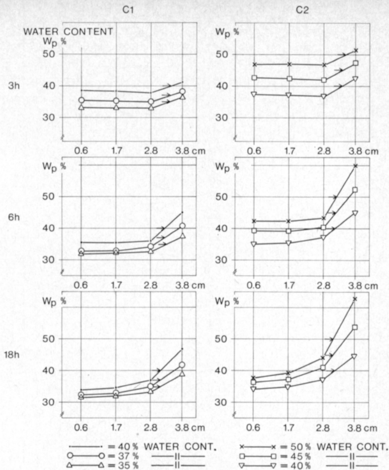
Fig. 13. Movement of soil water in the big C1— and C2— soil cylinders prepared from paste at three different soil water contents and three different freezing periods. The small arrow \rightarrow by the curve indicates the water content in the beginning of freezing. Freezing temperature -5^{\circ}\text{C} .
