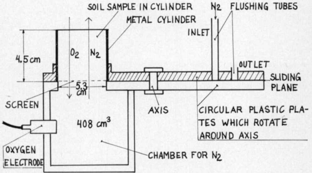
Fig. 6. Diagram of the apparatus used for determining the apparent diffusion coefficient. For filling of chamber with N 2 the upper disc is rotated 180°.
