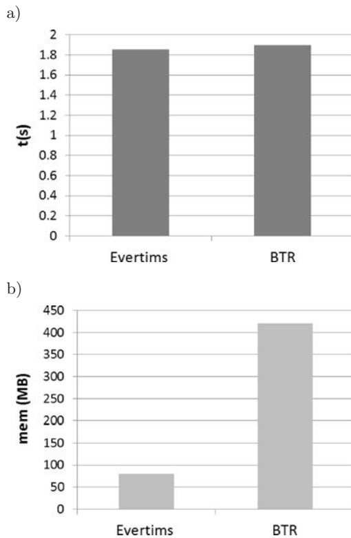
Fig. 13. The speed (a) and the memory consumption (b) of the simulation of Sigyn hall with Evertims and the BTR.
