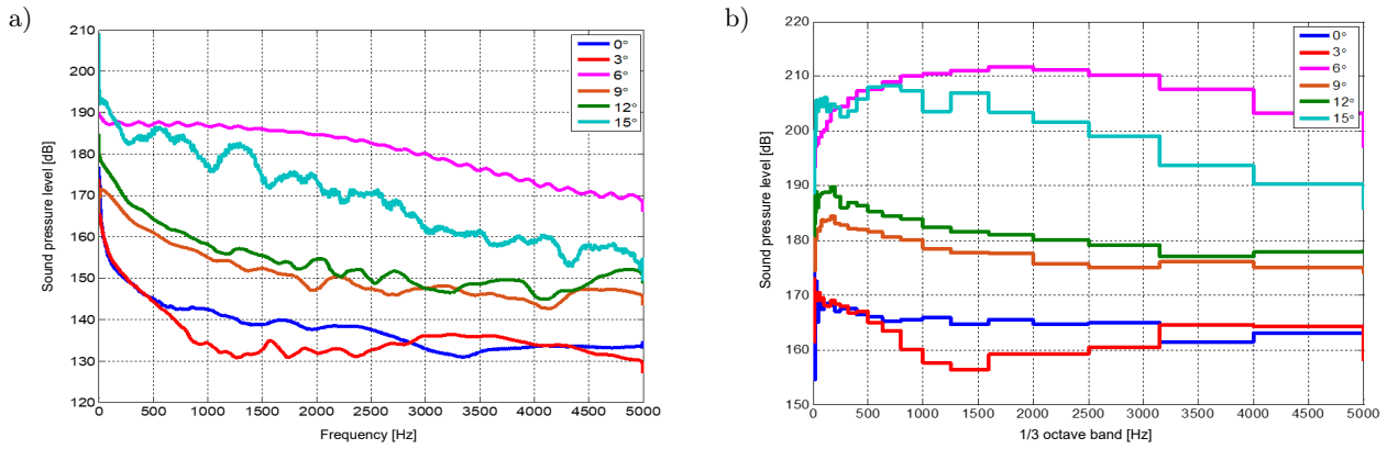
Fig. 19. Sound pressure frequency spectrum curves of R7 at 0°, 3°, 6°, 9°, 12°, 15°.
