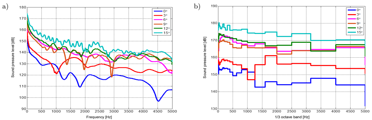
Fig. 13. Sound pressure frequency spectrum curves of R7 at 0°, 3°, 6°, 9°, 12°, 15°.
