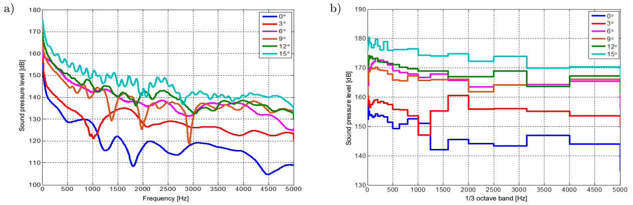
Fig. 11. Sound pressure frequency spectrum curves of R6 at 0°, 3°, 6°, 9°, 12°, 15°.
