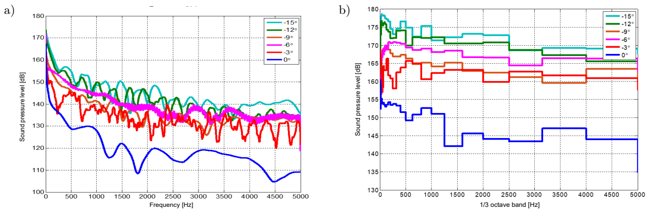
Fig. 12. Sound pressure frequency spectrum curves of R6 at 0°, -3°, -6°, -9°, -12°, -15°.
