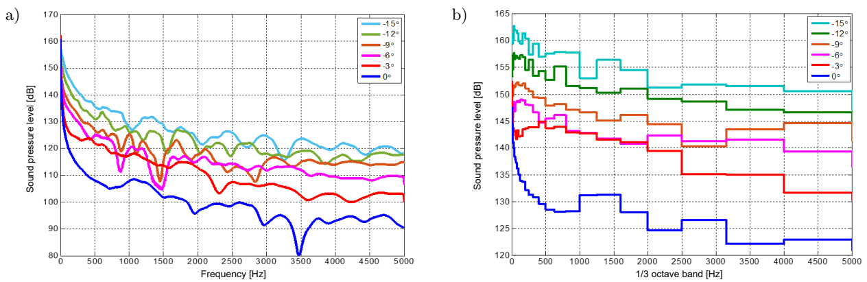
Fig. 4. Sound pressure frequency spectrum curves of R1 at 0^\circ, -3^\circ, -6^\circ, -9^\circ, -12^\circ, -15^\circ .
