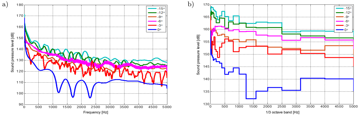
Fig. 10. Sound pressure frequency spectrum curves of R1 at 0°, -3°, -6°, -9°, -12°, -15°.
