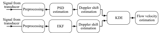
Fig. 6. Signal processing scheme.
