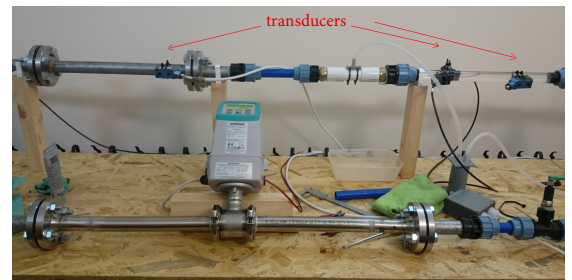
Fig. 7. Measurement equipment.
