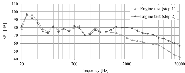
Fig. 13. Measured SPL inside the cabin; the engine test (steps 1 and 2).
