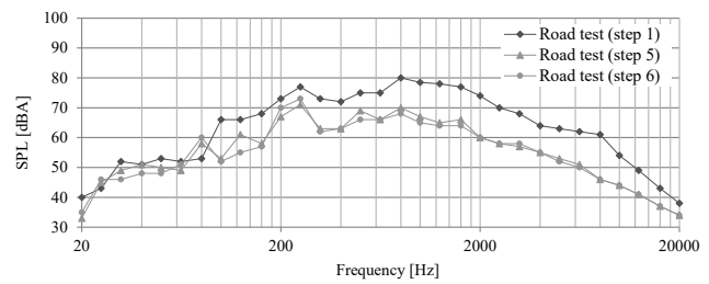
Fig. 15. Measured SPL inside the cabin; the road test (steps 1, 5, and 6) in dBA.
