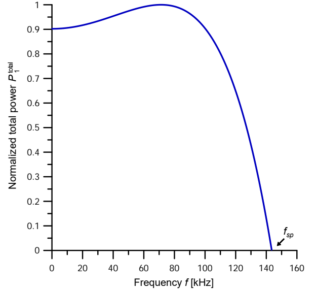
Fig. 6. Normalized total power P_1^{\text{total}} carried by the surface wave in the direction of propagation x_1 , as a function of wave frequency f . Surface resonant frequency f_{sp} = 143.569 kHz.
