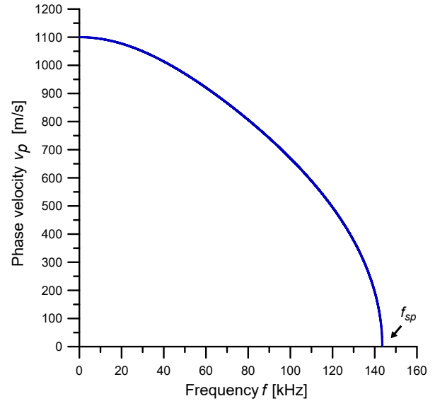
Fig. 3. Phase velocity v_p of the new surface wave versus frequency f . Note that, v_p(\omega \rightarrow 0) \rightarrow v_2 and v_p(\omega \rightarrow \omega_{sp}) \rightarrow 0 .
