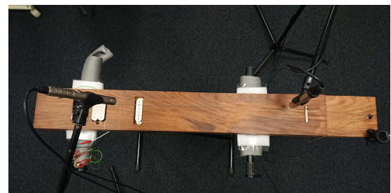
Fig. 2. Rosewood sample being set up for testing.
