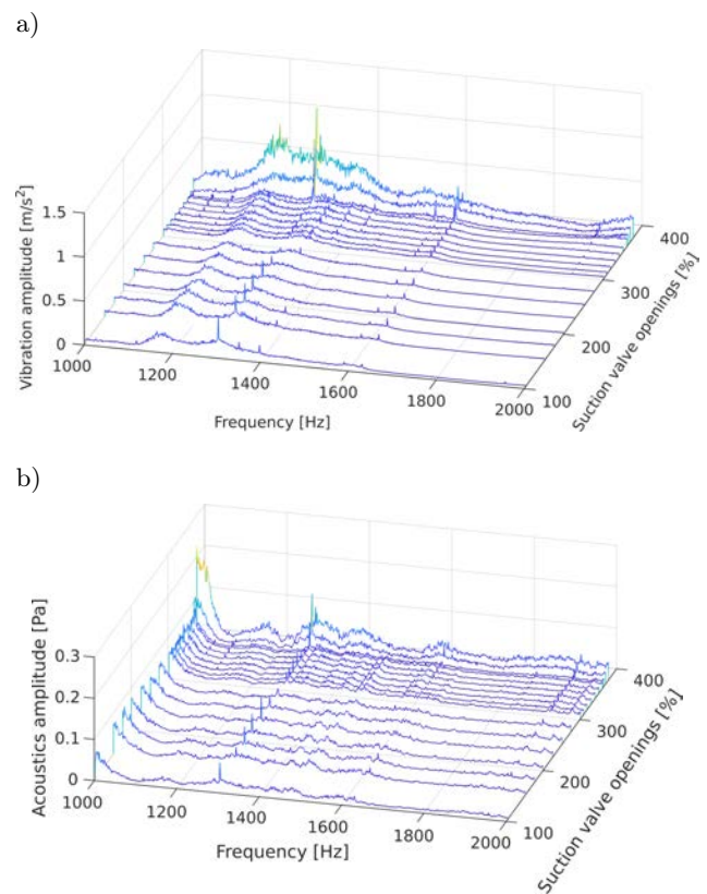
Fig. 10. Frequency domain under various flow rates and the frequency range from 1 kHz to 2 kHz at 2755 rpm.
