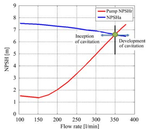
Fig. 4. The cavitation characteristics of the centrifugal pump under different flow rates.
