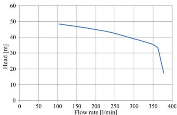
Fig. 3. Head of the centrifugal pump under pump rotational speed 2755 rpm.
