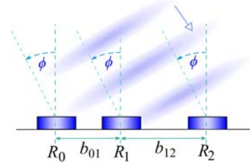
Fig. 7. Two pairs of receivers integrated into a single system of three transducers.
