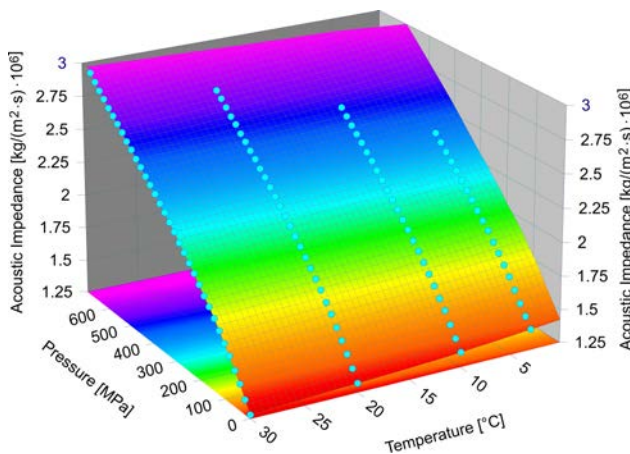
Fig. 6. Acoustic impedance Z_a of the low-pressure phase of the Camelina sativa oil, as a function of pressure p and temperature T .
