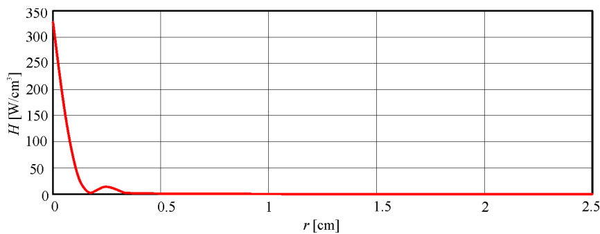
Fig. 6. Radial power in the ultrasonic radiation focus.
