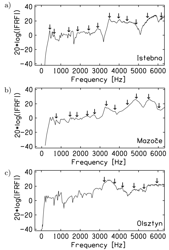
Fig. 1. Examples of the FRFs measured on spruce samples of: a) subjectively evaluated as a good quality resonance wood (Istebna), b) subjectively evaluated as a high quality resonance wood (Mazoče), c) non-resonance wood (Olsztyn). Arrows indicate frequencies of modes described in the text.
