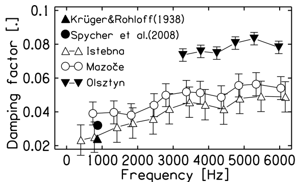
Fig. 2. Relation between the damping factor and modal frequencies of spruce wood samples of resonance (Istebna and Mazoče) and non-resonance spruce wood (Olsztyn). Vertical bars indicate single standard deviation. Data of KRÜGER and ROHLOFF (1938) and SPYCHER et al. (2008) are shown for comparison.
