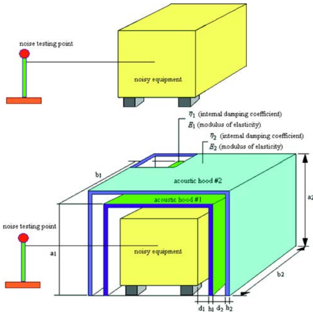
Fig. 1. The noise testing point for a two-layer close-fitting acoustic hood.
