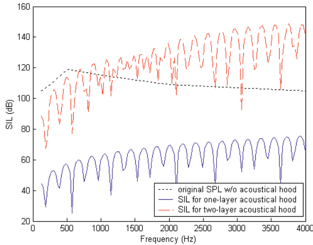
Fig. 10. Comparison of the original SPL and an optimal SIL for a two-layer close-fitting acoustic hood (broadband noise).
