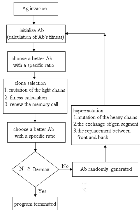
Fig. 4. The flow diagram of the artificial immune method.
