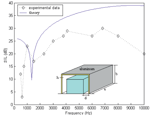
Fig. 2. The performance curve with respect to the theoretical and experimental data [ a = b = 0.293 (m); \eta = 0.33 ; d = 0.012 (m); h = 0.013 (m)] (BLANKS, 1997).
