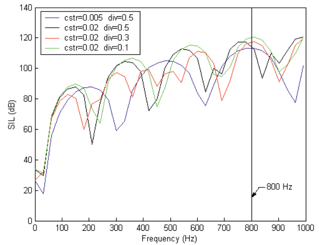
Fig. 8. The SIL with respect to frequencies at various AIM parameters ( cstr , iter ) (targeted tone: 800 Hz).
